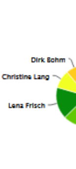
Top 5 Agents
